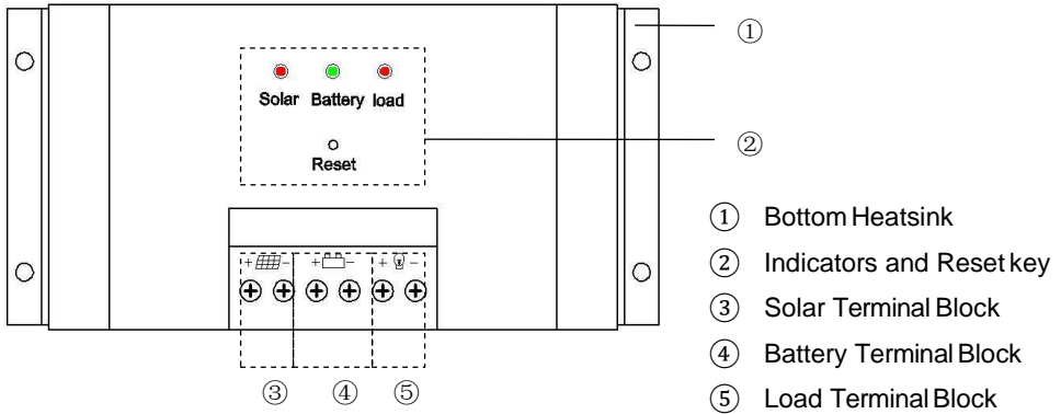
Figure 2-1: Controller Structure Diagram
