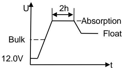
Figure 2-2: Three-stage Charge
