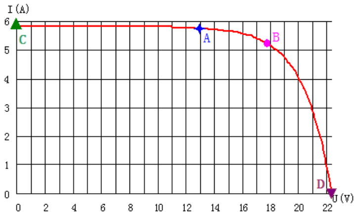
Figure 2-4: Voltage-Current Curve
