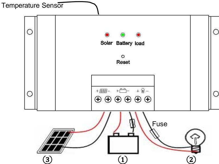
Figure 4-2: Connecting Diagram
