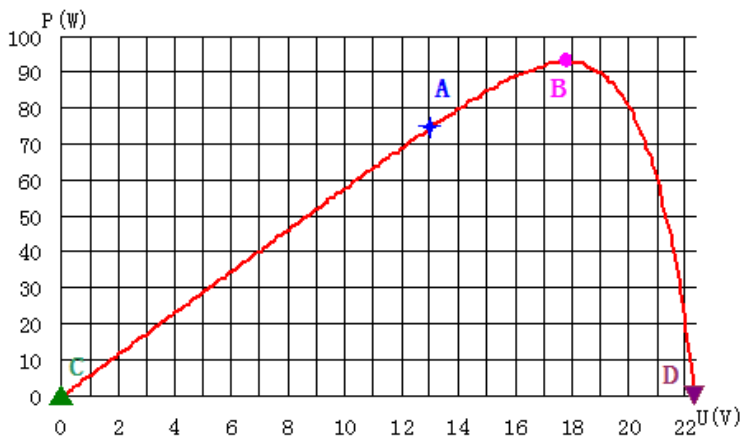
Figure 2-5: Voltage-Power Curve
