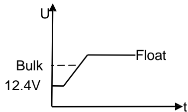
Figure 2-3: Two-stage Charge
