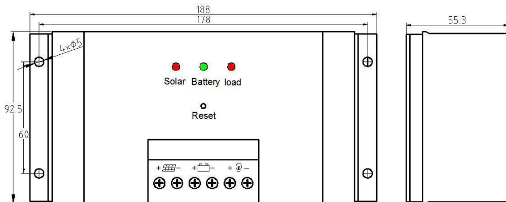
Figure 4-1: Dimensions (Unit: mm)
