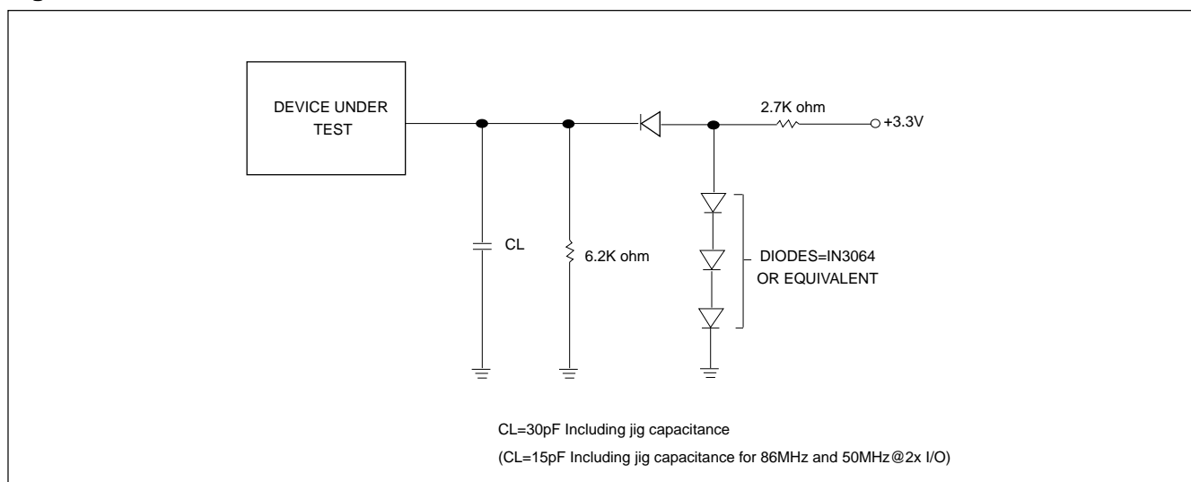
Figure 7. OUTPUT LOADING
