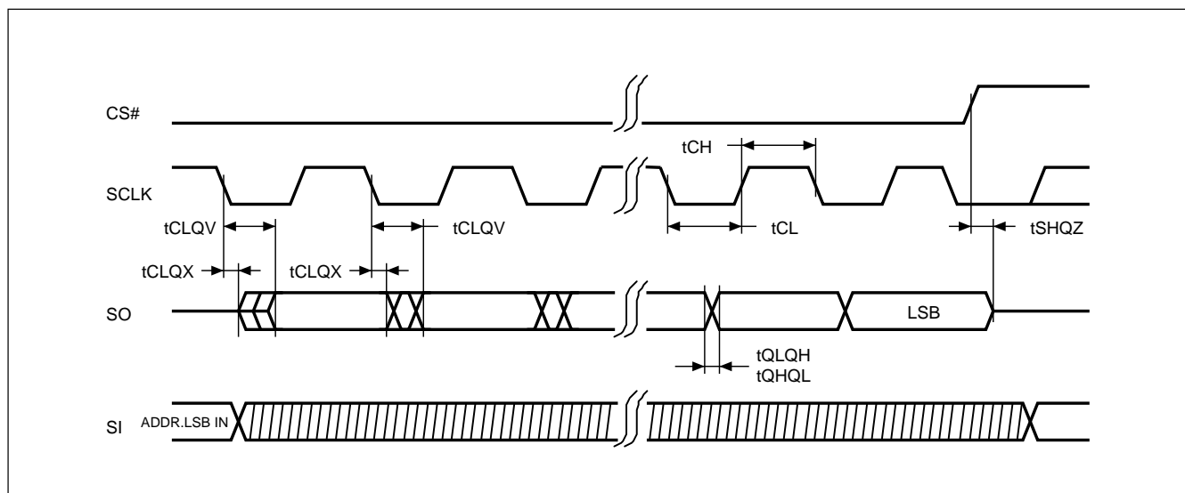
Figure 9. Output Timing
