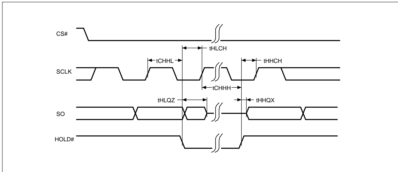
Figure 10. Hold Timing
