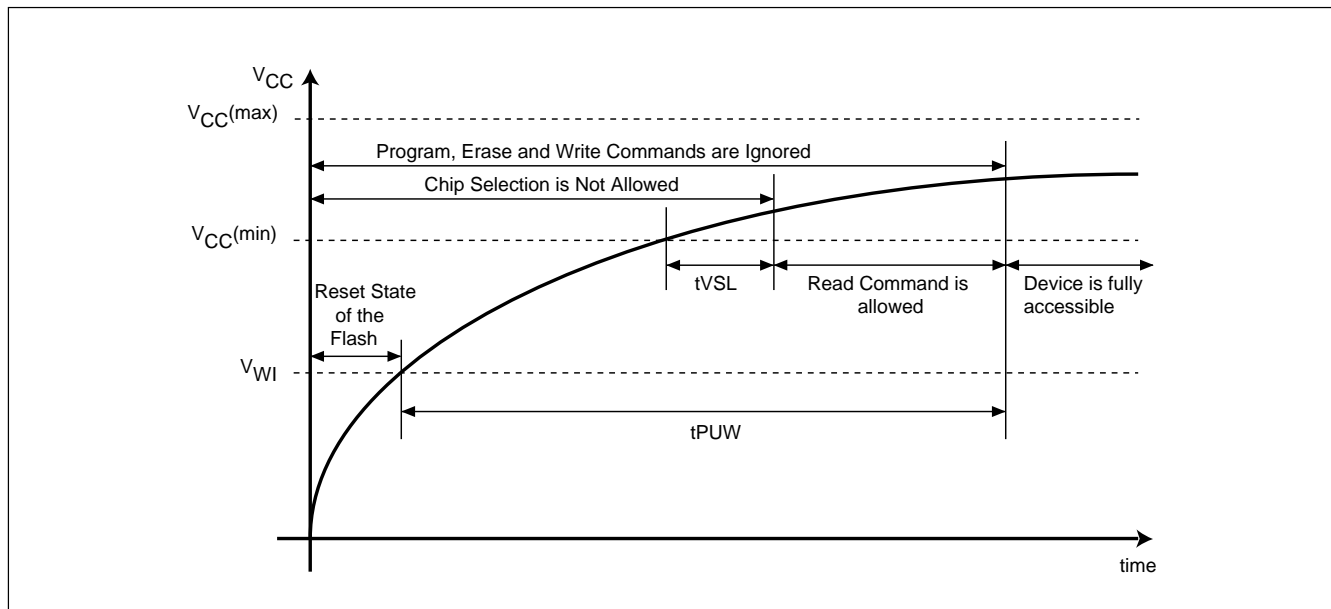
Figure 29. Power-up Timing
