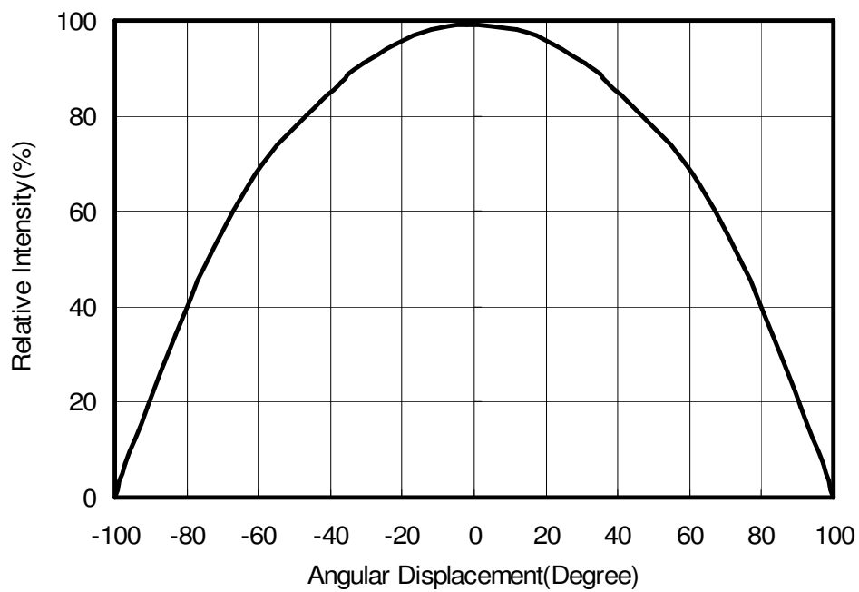
< Figure 10.Lambertain at T_J=25^{\circ}\text{C} for blue and true green >
