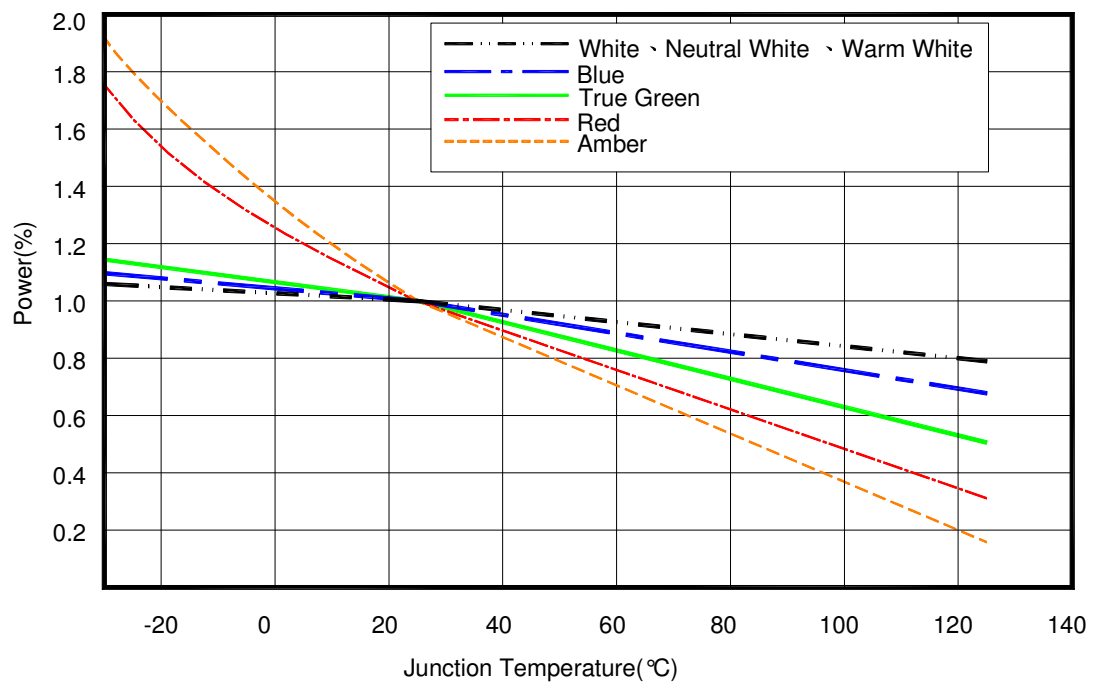
< Figure 28. Junction temperature & power rate for Edixeon® series >
