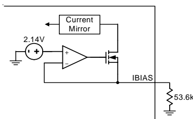
Figure 4. IBIAS Setting
