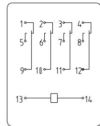
(Bottom View)底视
