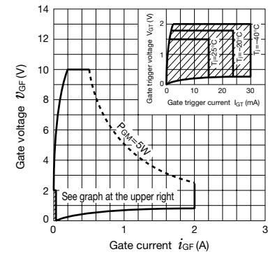
Gate Characteristics
