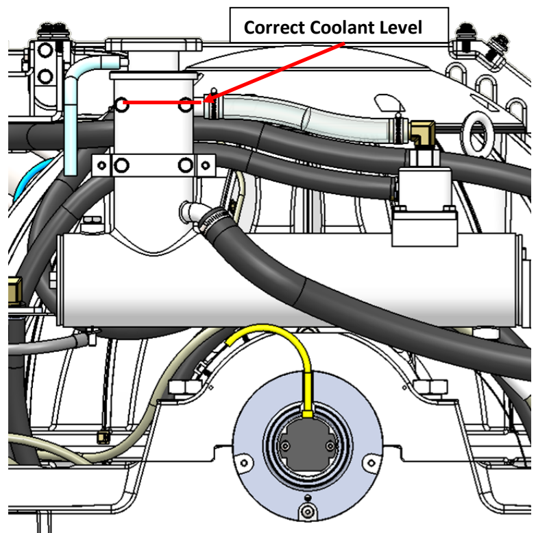
FIGURE 3 – SEAKEEPER 9 COOLANT LEVEL
