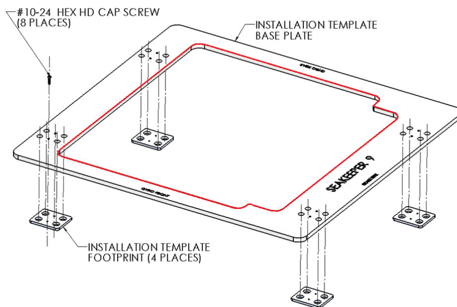
FIGURE 5 – EXPLODED VIEW OF INSTALLATION FIXTURE
