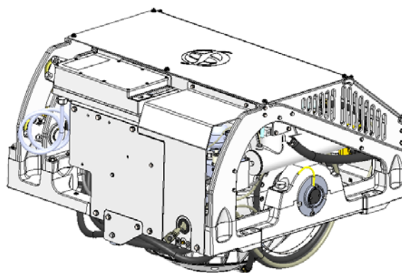
SEAKEEPER 9 Gyro, Rear Oblique View
