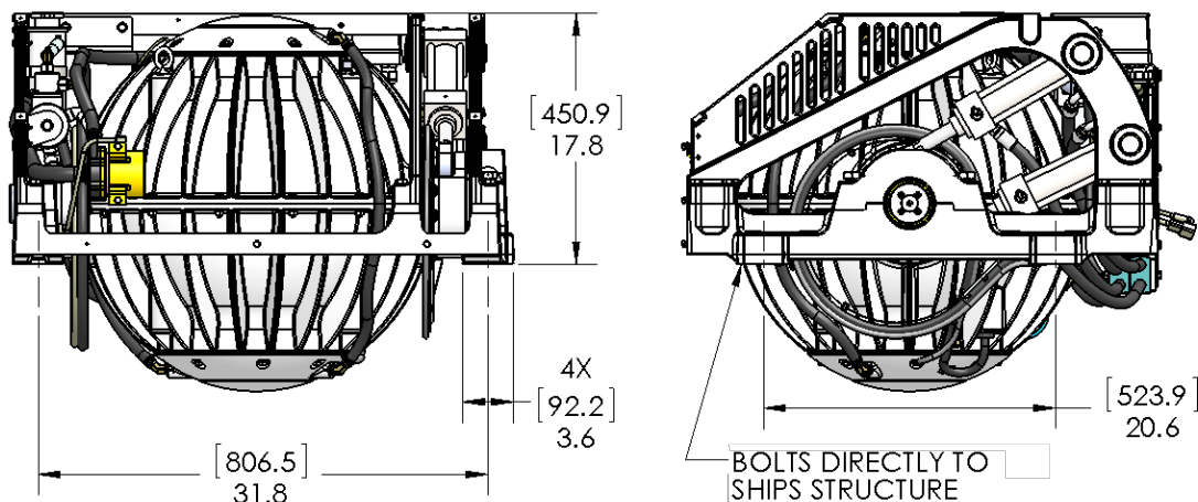
OPTION 1- DIRECT FASTENING OF GYRO FOUNDATION TO SHIPS STRUCTURE
