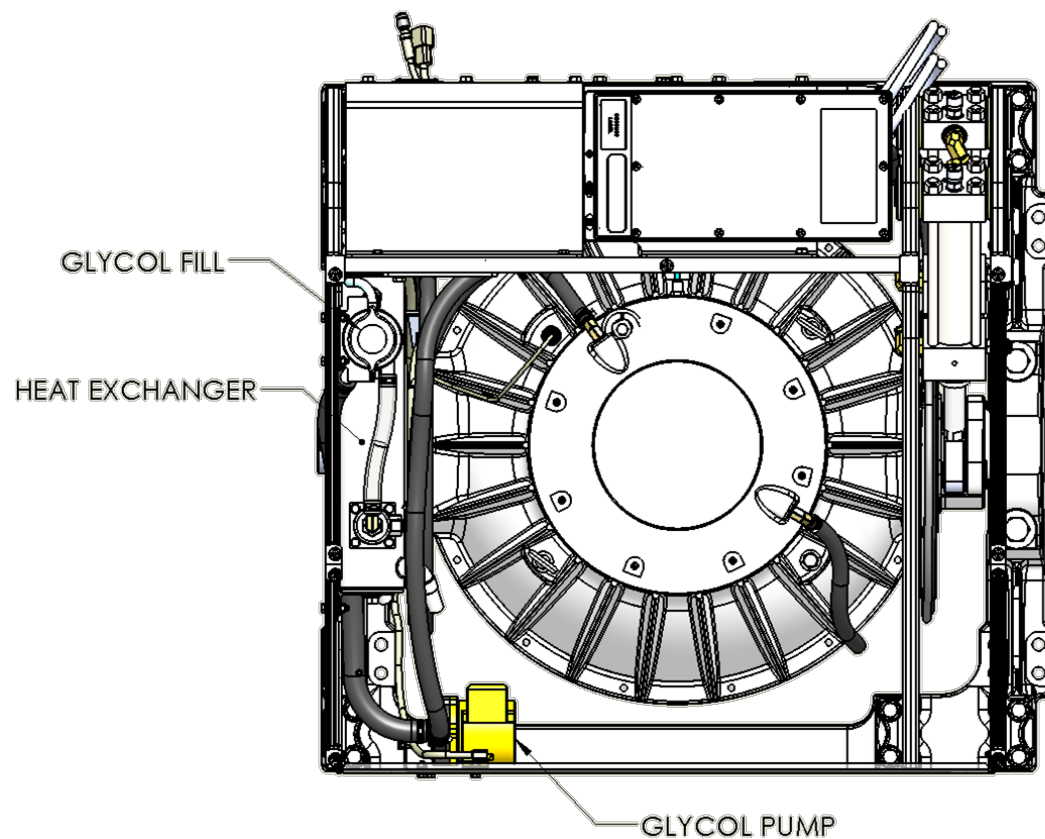
FIGURE 1 – SEAKEEPER 9 GYRO
