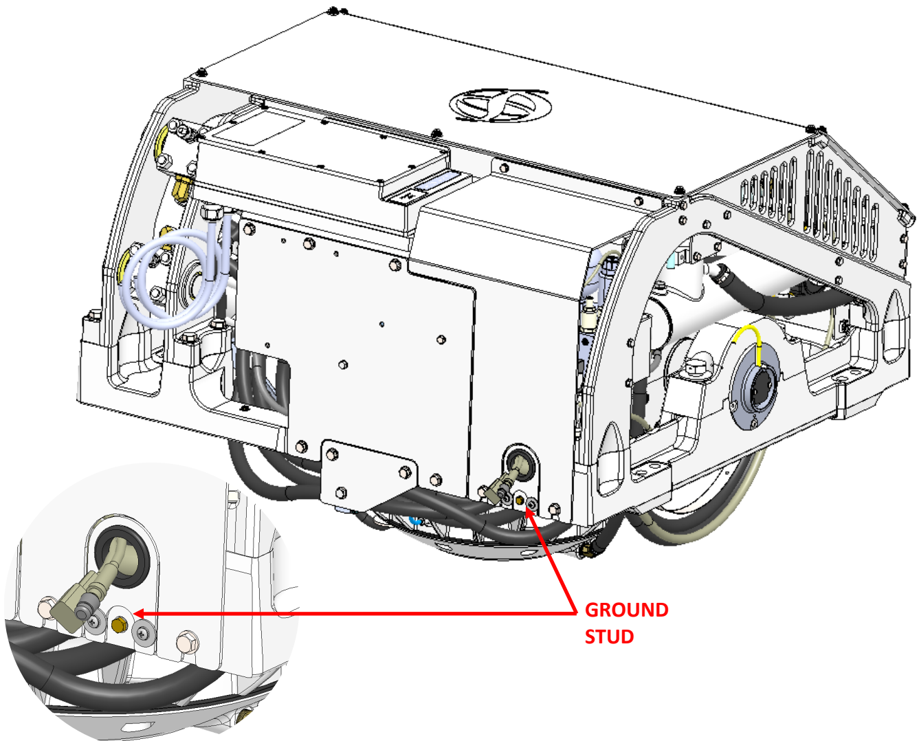
FIGURE 9 – GYRO GROUND STUD ON REAR BRACE
