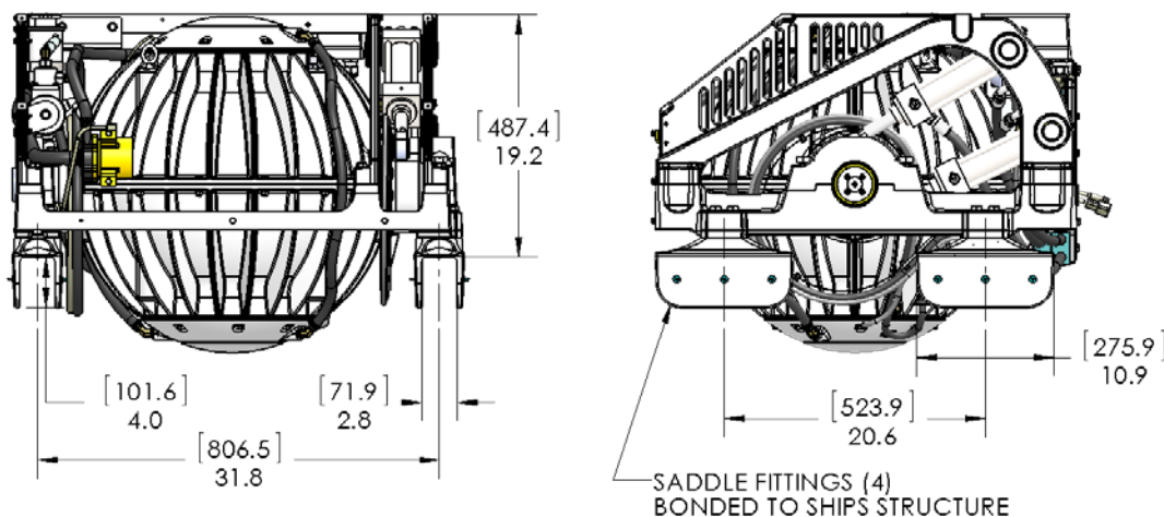
OPTION 2- SADDLE INSTALLATION (4 PLACES)
