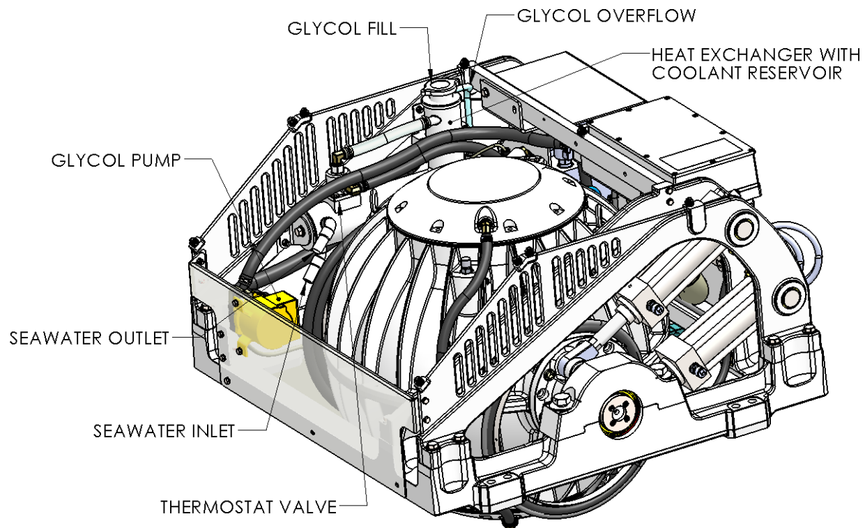
FIGURE 4 – SEAKEEPER 9 SEAWATER CONNECTIONS
