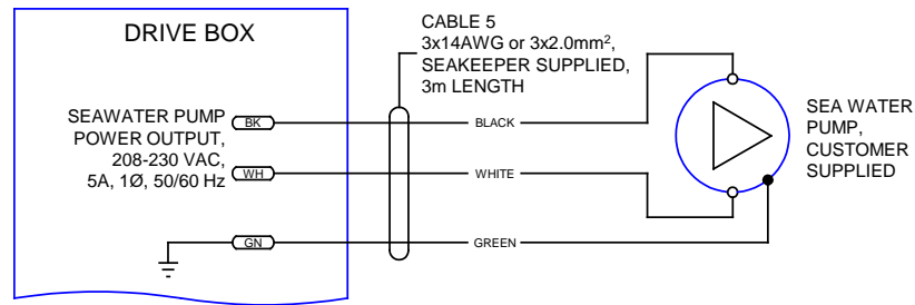
FIGURE 5 – CABLE 5, WIRE CONNECTIONS TO SEAWATER PUMP
