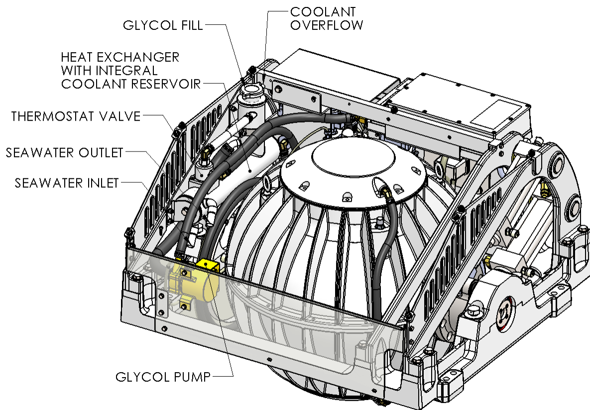
FIGURE 2 – SEAKEEPER 9 GYRO COOLING COMPONENTS
