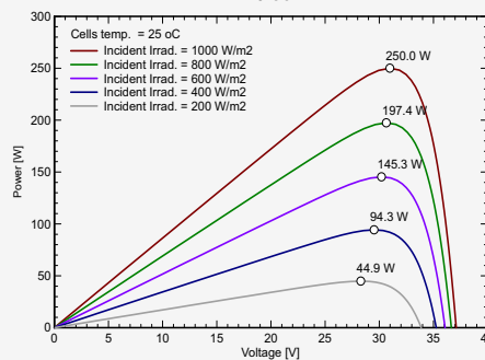
STC: Irradiance 1000W/m 2 , Module temperature 25°C, AM1.5 spectrum.
