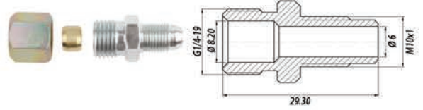
Nipel Set M10 x 1 / G1/4 - 19 Metal Nipple Set M10 x 1 / G1/4 - 19 Metal
