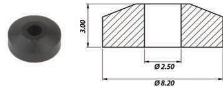
Conta Şamandıra Vana Pim Gasket for Multivalve Pin
