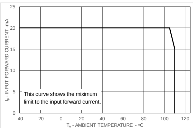
Figure 2. I_F vs. Temperature
