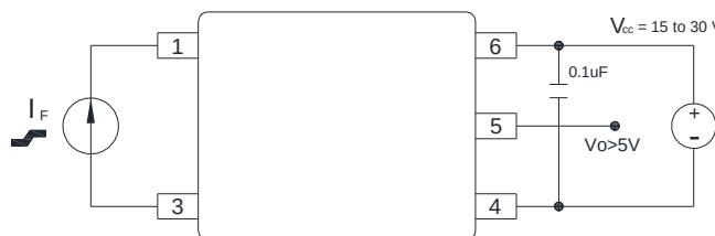
Figure 18 : I_{FLH} Test Circuit
