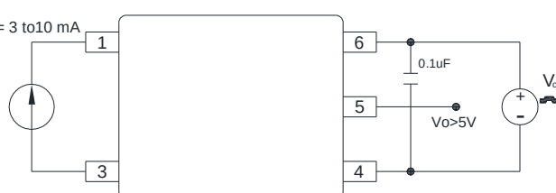
Figure 19 : U_{VLO} Test Circuit
