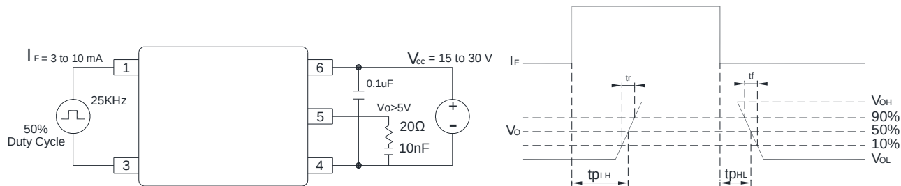
Figure 20 : t_r , t_f , t_{PLH} and t_{PHL} Test Circuit and Waveforms
