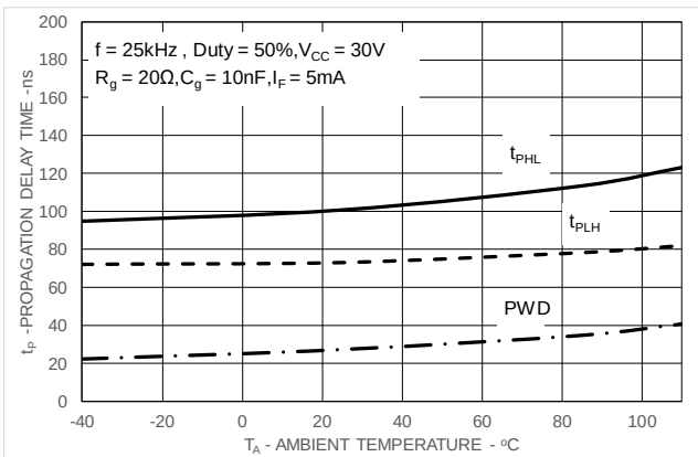
Figure 11. Propagation Delay Time vs. Temperature
