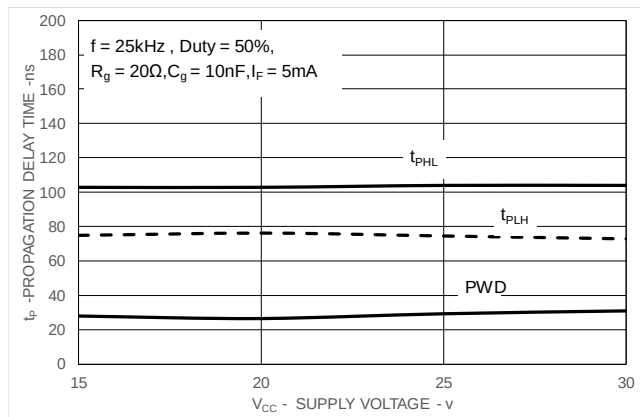
Figure 13. Propagation Delay Time vs. V_{CC}
