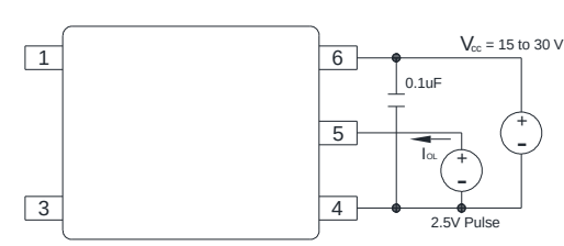
Figure 17 : I_{OL} Test Circuit
