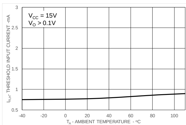
Figure 4. I_{FLH} vs. Temperature
