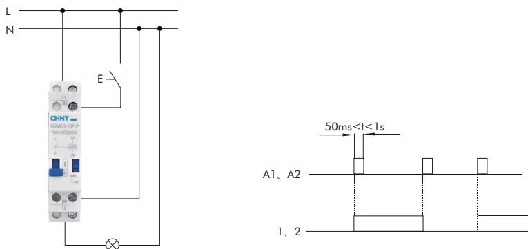
Connection diagram and sequence chart
