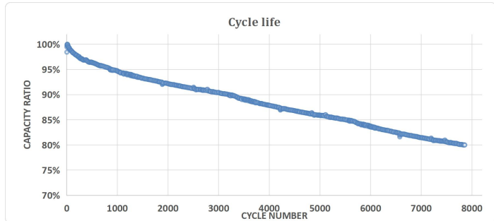
Curve of cyclelife
