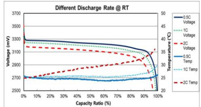
Curve of different discharge rate
