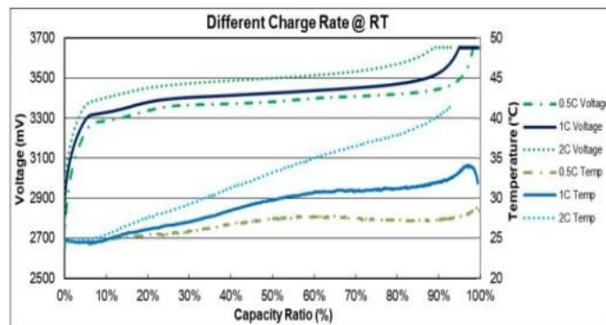
Curve of different charge rate
