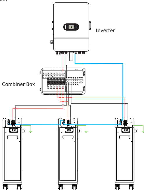
Figure 4-1 The parallel connection of three battery packs
