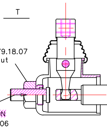
P80 directional control valve
