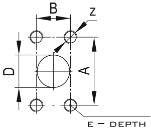
D – SAE FLANGE (UNC)
