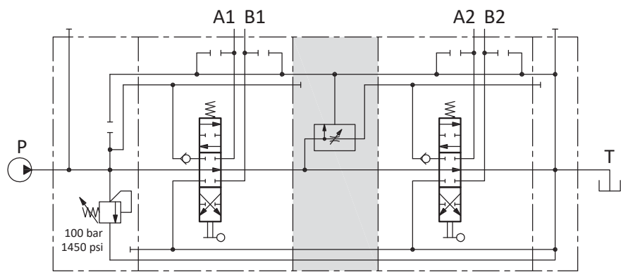
Hydraulic circuit
