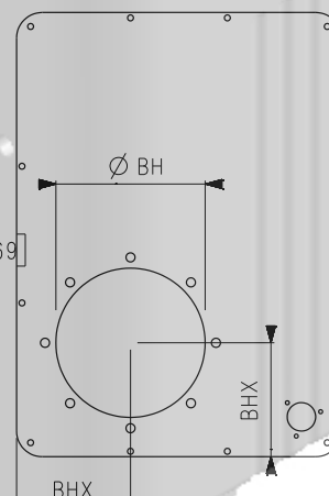
Style C Lid plate with Filler Breather (FB) and Bellhousing (BH) cutout Lid
