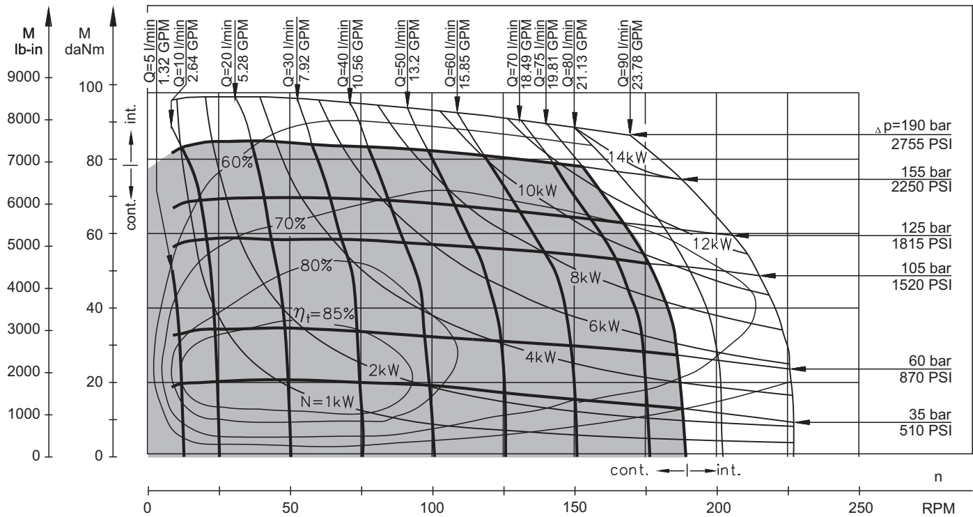
MH 400
