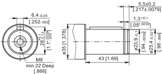
CO - \varnothing 1" straight, Parallel key \frac{1}{4}" \times \frac{1}{4}" \times 1\frac{1}{4}" BS46 Max. Torque 34 daNm [3010 lb-in]
