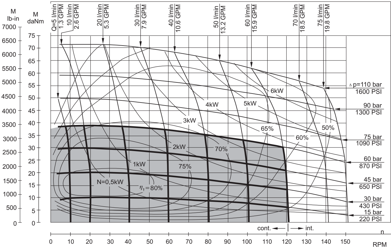
MP 500
