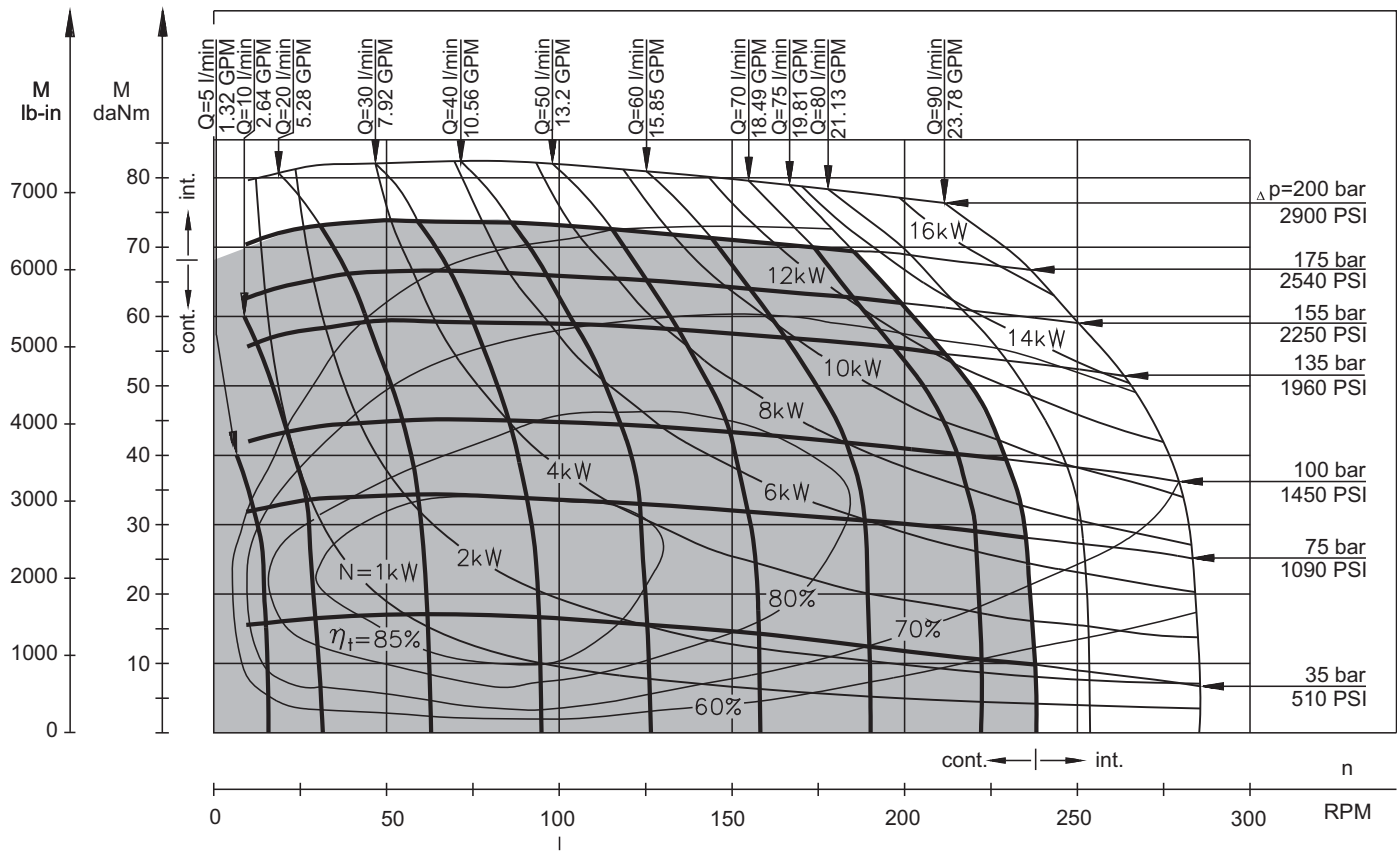
MH 400
