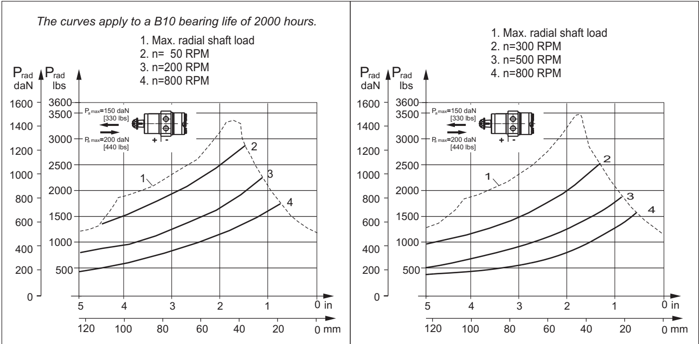
MPWN
