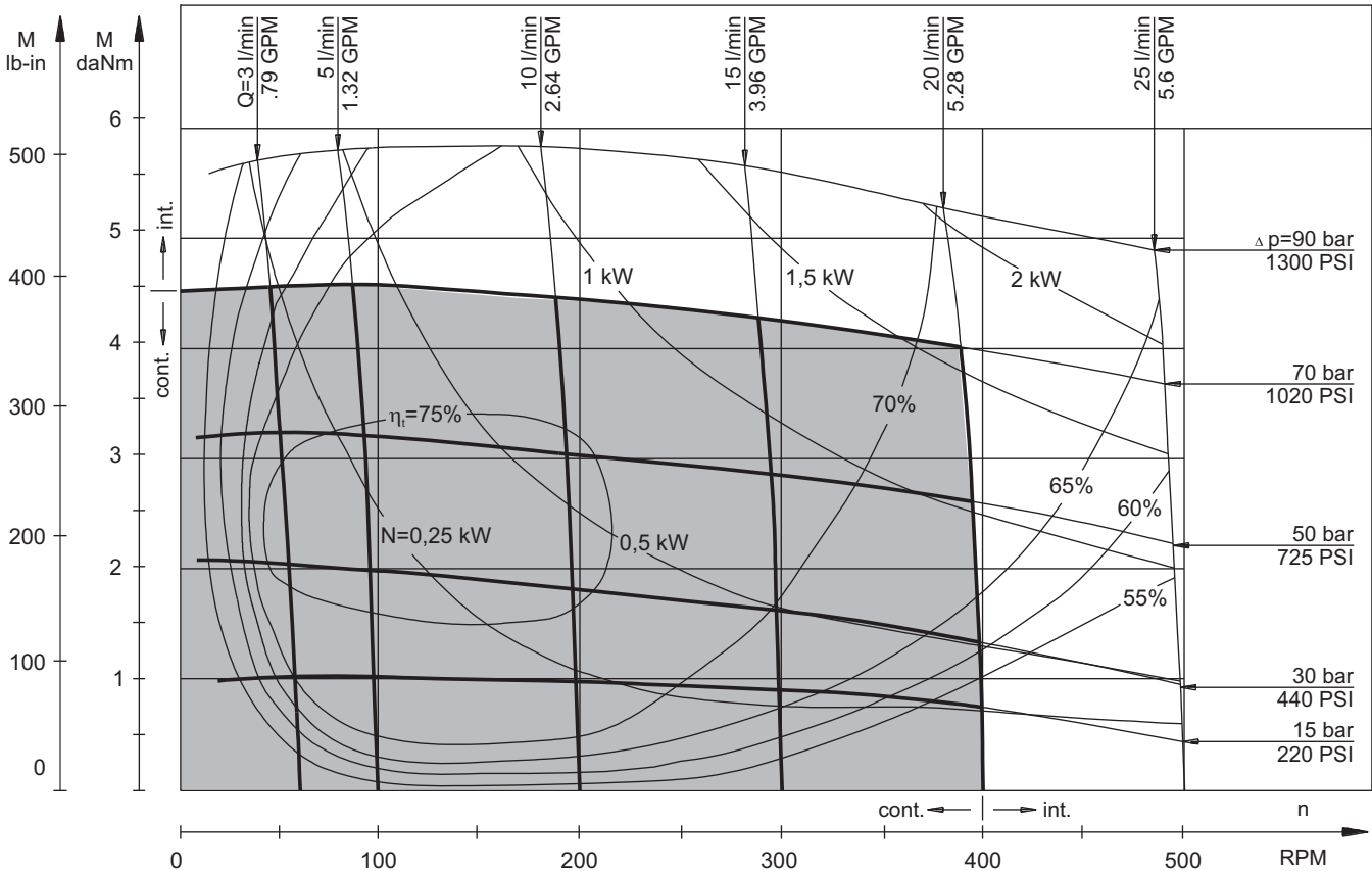
MM 50
