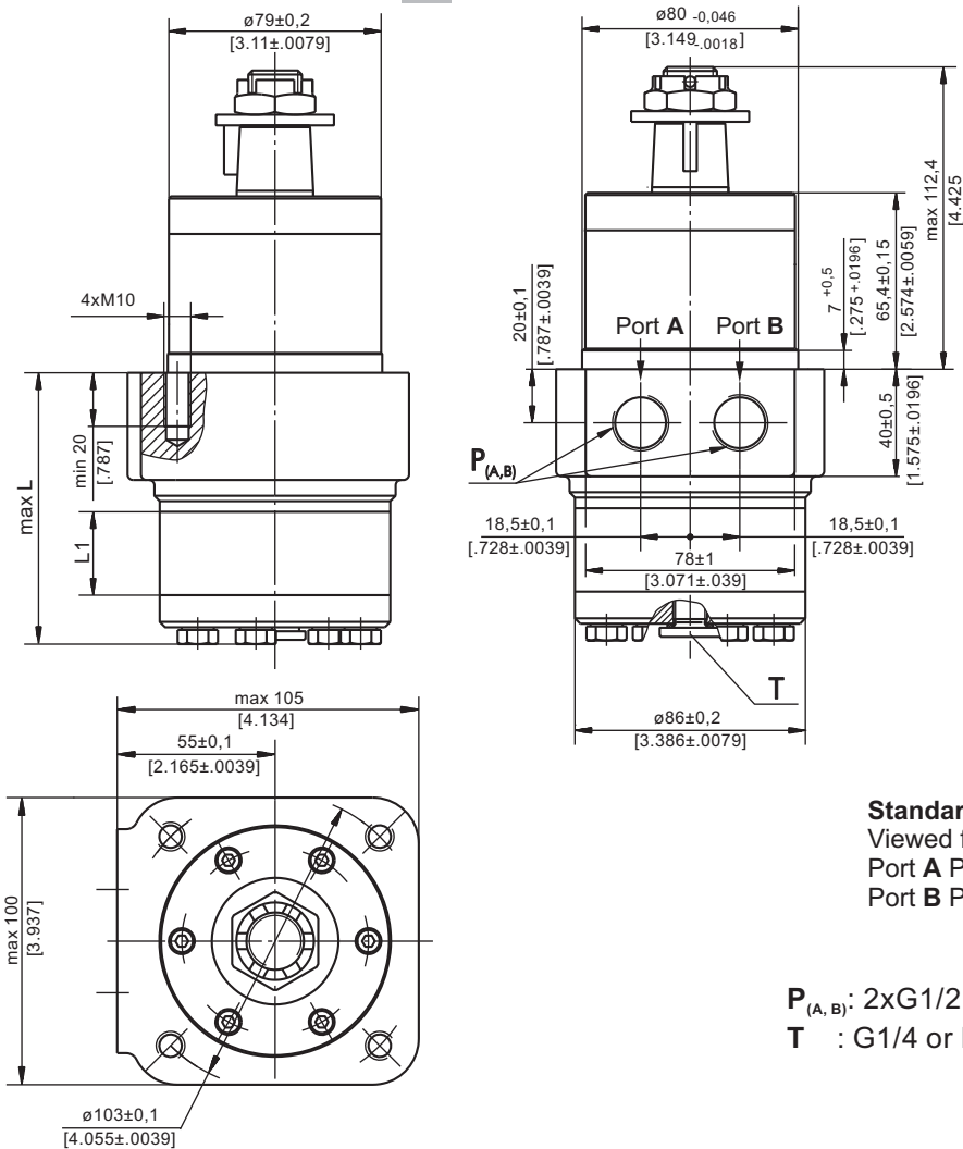
MPWN
