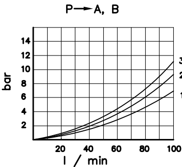
operating diagrams
