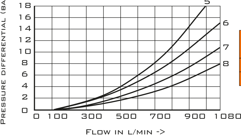
\Delta P-Q_v CHARACTERISTIC CURVES – SYMBOL G AND T
