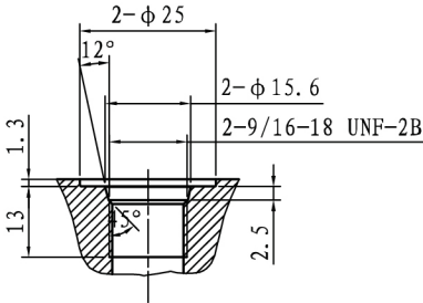
Sectional view of A,B oil port SAE8 1.5:1
