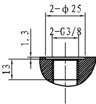
Sectional view of A,B oil port G3/8
