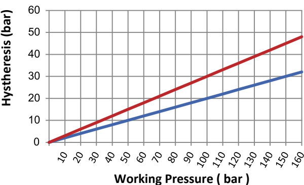
Pressure Set Range 10 ... 160 bar max set pressure 160 bar max system pressure 650 bar
