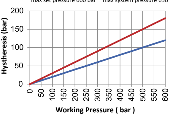
Pressure Set Range 50 ... 600 bar max set pressure 600 bar max system pressure 650 bar
