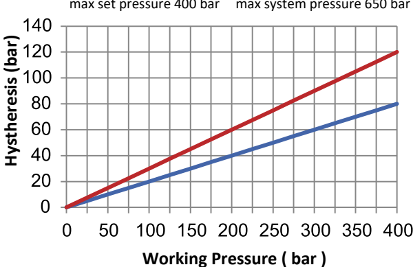
Pressure Set Range 20 ... 400 bar max set pressure 400 bar max system pressure 650 bar
