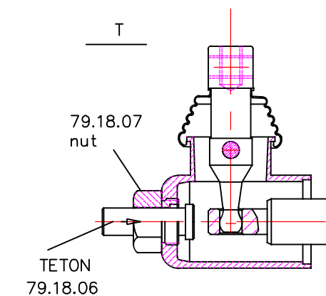
P40 directional control valve
