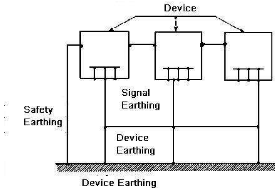
Appendix Figure 7-2 Multiple-point ground
