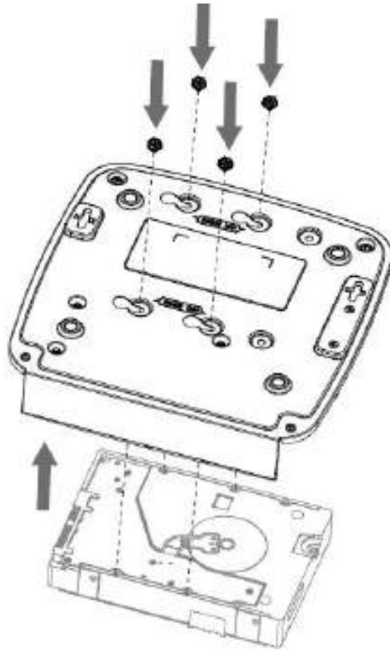
Figure 2-32 Install HDD
