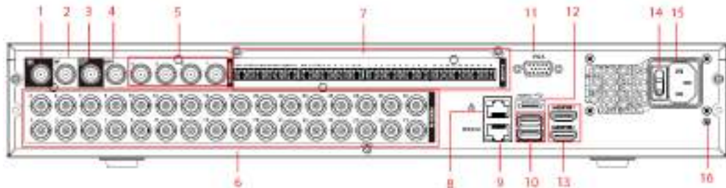
Figure 3-20 Rear panel (2)
