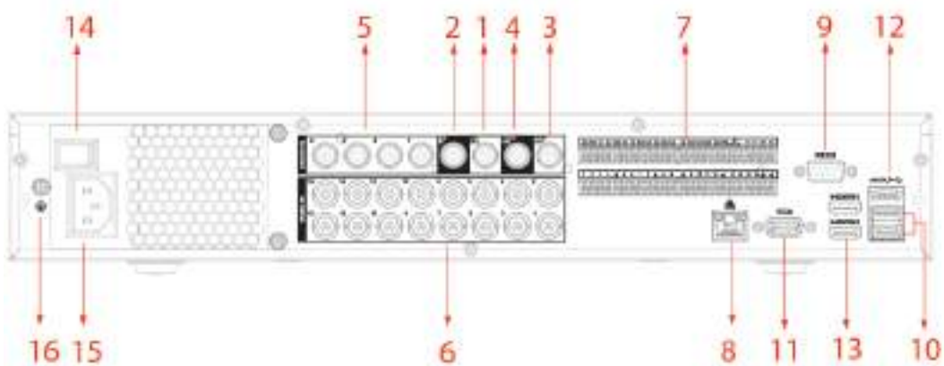
Figure 3-21 Rear panel (3)
