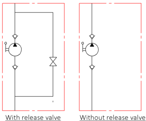
Hydraulic schemes
