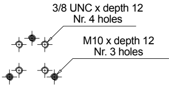
Fixing holes Option for Metric and UNC screws
