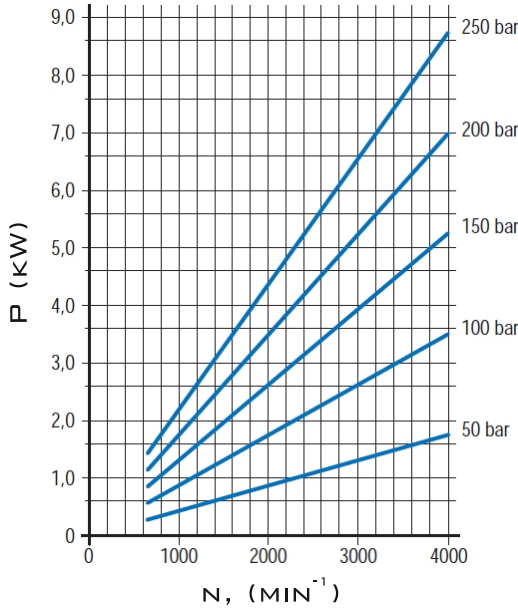
MGP1K4.2
