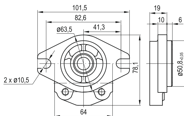
30 - SAE "A-A" 2 BOLTS
