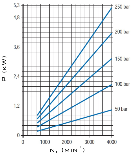
MGP1K2.5
