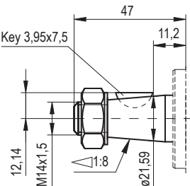
G3 - EUROPEAN TAPERED 1:8
