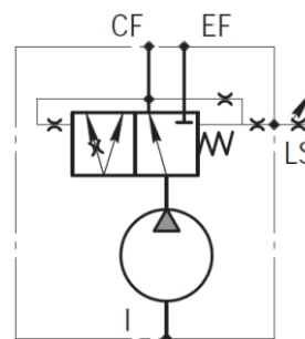
VPLD – PRIORITY VALVE WITH DYNAMIC LS CONTROL
