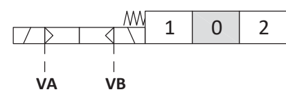
Scheme ISO 1219
