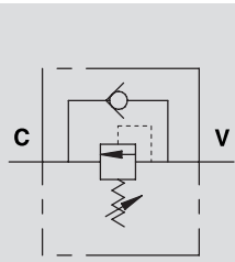
SCHEMA IDRAULICO HYDRAULIC DIAGRAM
