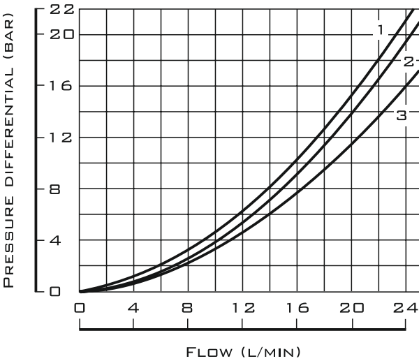
\Delta P -Q CHARACTERISTIC CURVES 3/2 DIRECTIONAL SEAT VALVE
