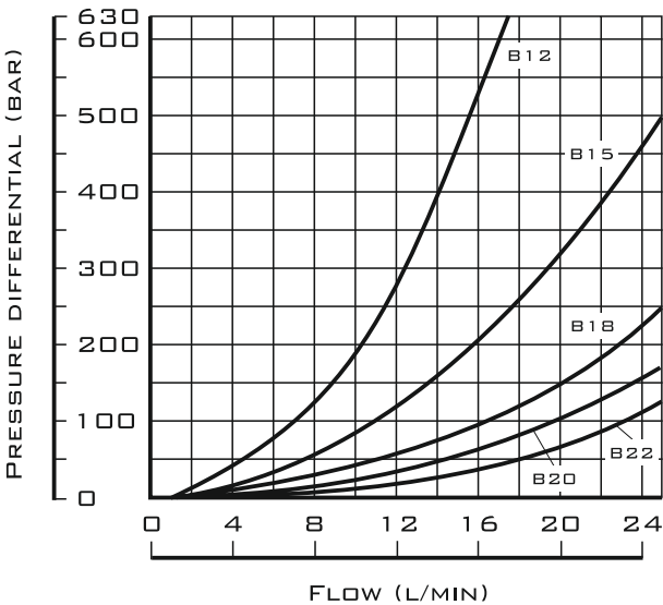
ΔP-Q CHARACTERISTIC CURVES THROTTLE INSERT
