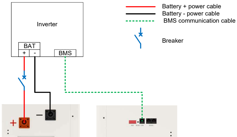
Fig. 4-1 Single MOON16-G Pro PACK + single inverter diagram
