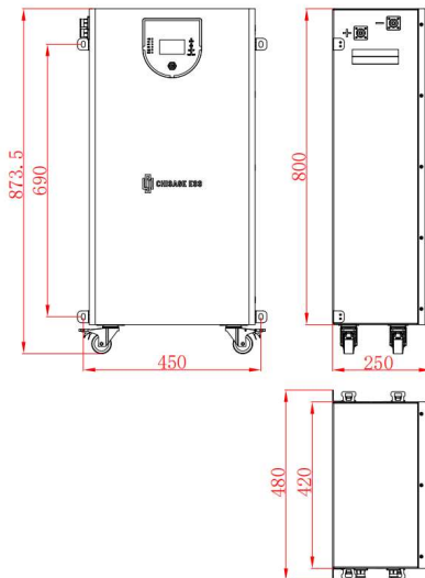
Fig. 3-2 MOON16-G Pro PACK dimension drawing
