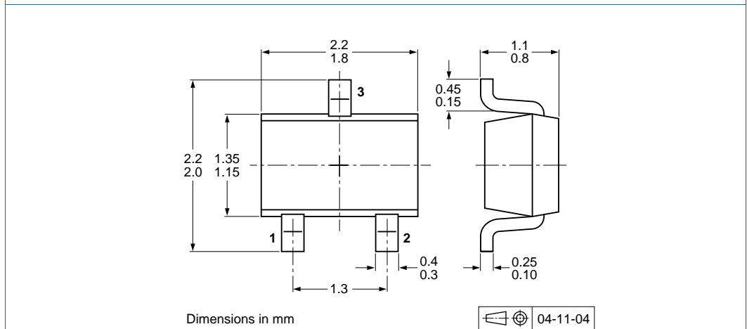
Fig 14. Package outline SOT323 (SC-70)
