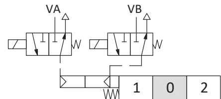
Scheme ISO 1219
