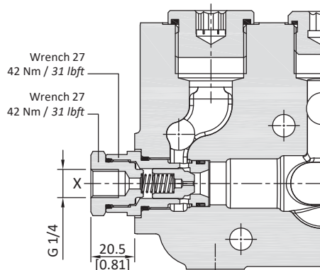
Hydraulic operated
