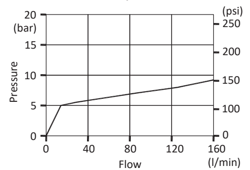
Pressure drop curve P → T
