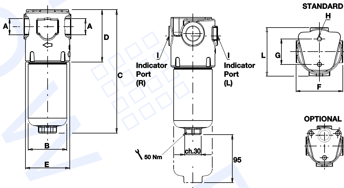
HIGH PRESSURE COMPLETE FILTER 280 bar
