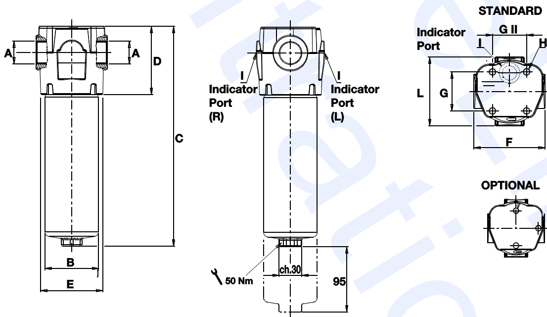
HIGH PRESSURE COMPLETE FILTER 280 bar
