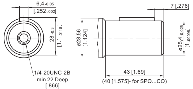
CO - \varnothing 1 " straight, Parallel key \frac{1}{4} "x \frac{1}{4} "x1" BS46 Max. Torque 34 daNm [3010 lb-in]
