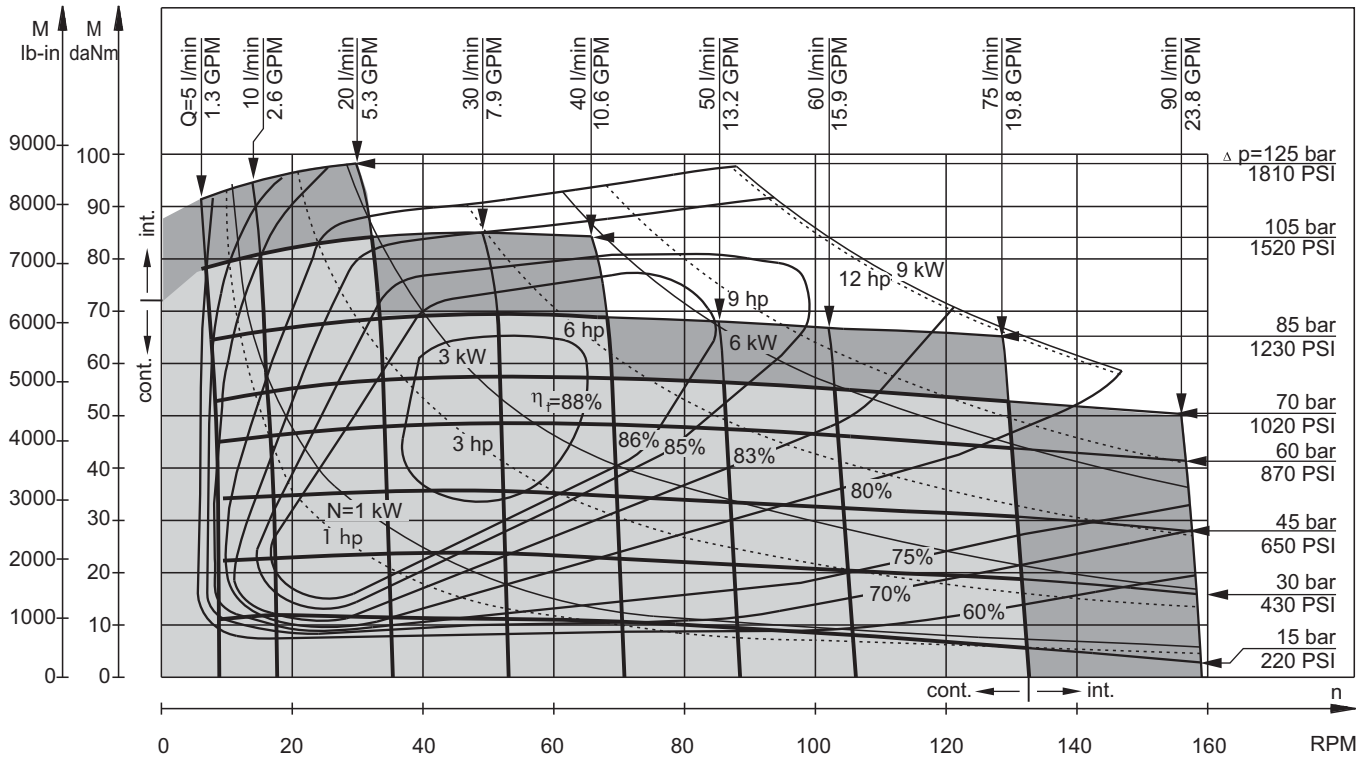
The function diagrams data is for average performance of randomly selected motors at back pressure 5÷10 bar [72.5÷145 PSI] and oil with viscosity of 32 mm²/s [150 SUS] at 50°C [122°F].
