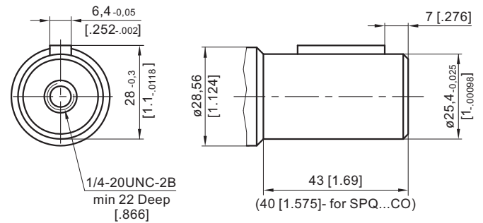
CO - \phi 1" straight, Parallel key \frac{1}{4}" \times \frac{1}{4}" \times 1" BS46 Max. Torque 34 daNm [3010 lb-in]
