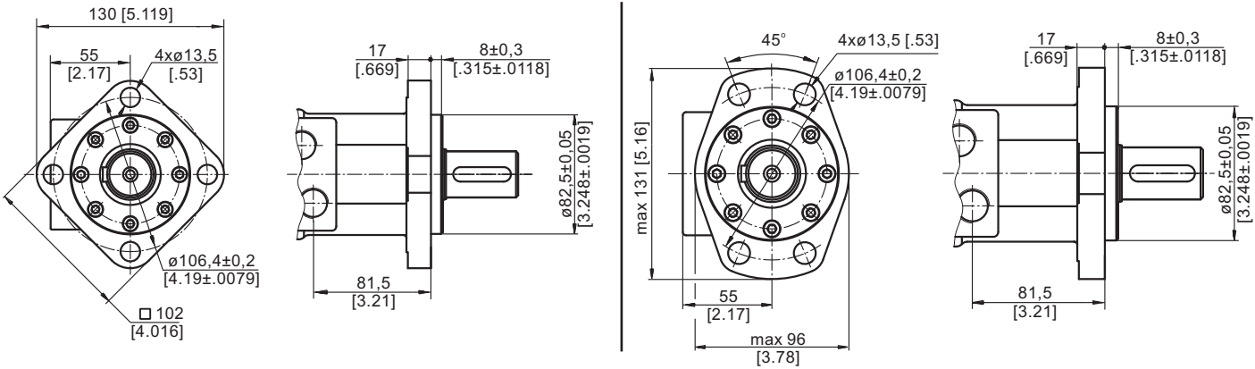
Square Mount (4 Holes)
