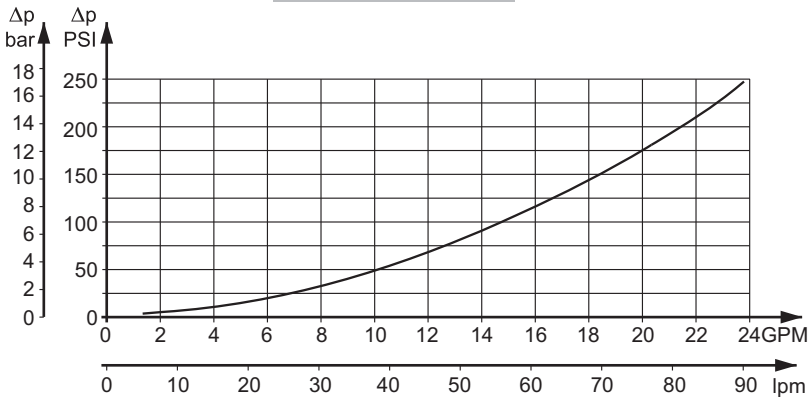
Pressure Losses
