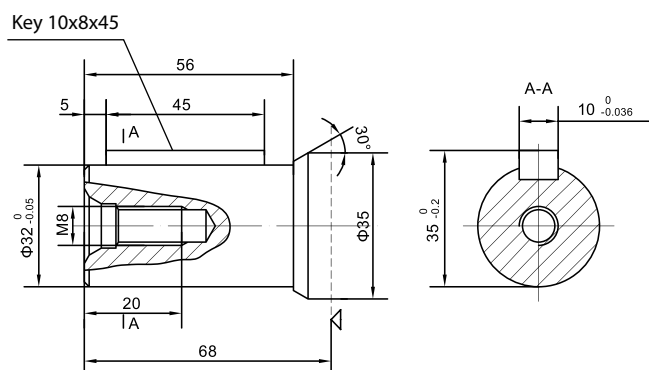
P52: Ø32 STRAIGHT SHAFT, PARALLEL KEY 10x8x45
