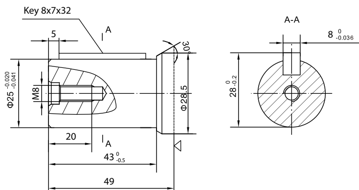
P4: Ø25 STRAIGHT SHAFT, PARALLEL KEY 8x7x32
