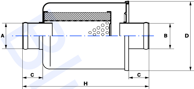
IN-LINE SUCTION FILTERS
