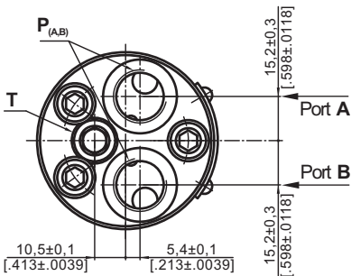
Rear Ports
