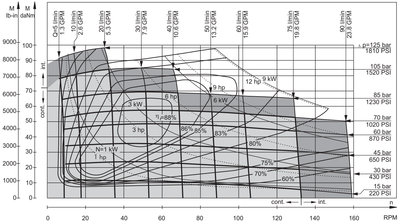
The function diagrams data is for average performance of randomly selected motors at back pressure 5÷10 bar [72.5÷145 PSI] and oil with viscosity of 32 mm 2 /s [150 SUS] at 50°C [122°F].
