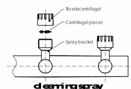
Cleaning condenser
