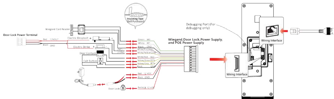
Figure 3-1 Terminal Diagram
