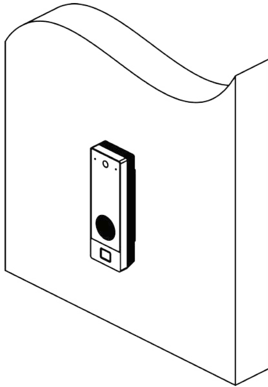
Figure 2-7 Complete Installation
