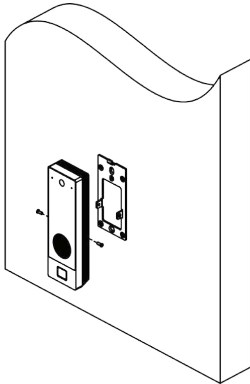
Figure 2-6 Secure Device
