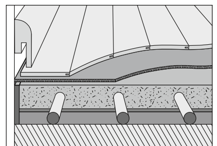
Engineered wood on Akustik-Protect underlay with hot water underfloor heating system
