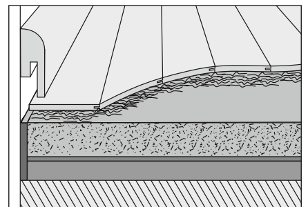
Engineered wood glued over the whole area
