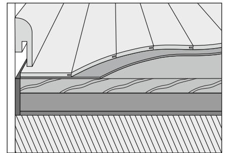
Engineered wood on Akustik-Protect 80 underlay / floorboards
