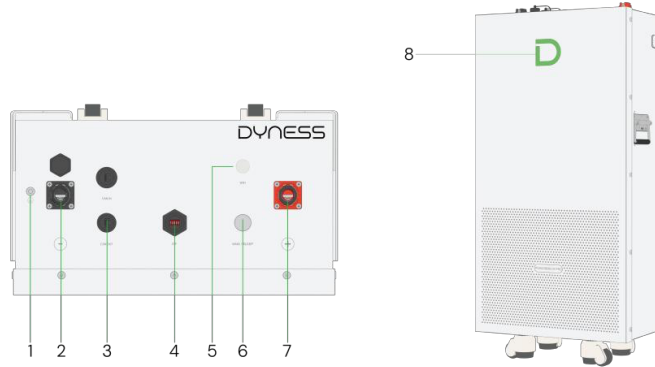
Figure 2-1 PowerBrick PLUS the Sketch of Front Interface
