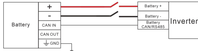
Figure 3-5 Wiring diagram
