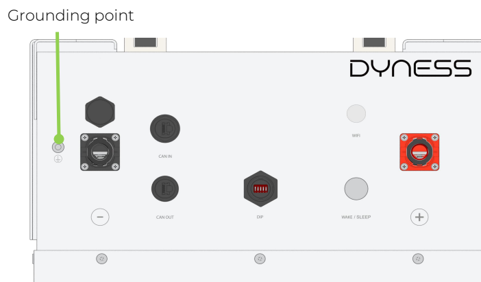
Figure 3-4 Location of grounding point
