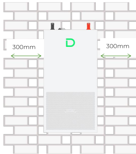
Figure 3-3 Mounting Space Requirements
